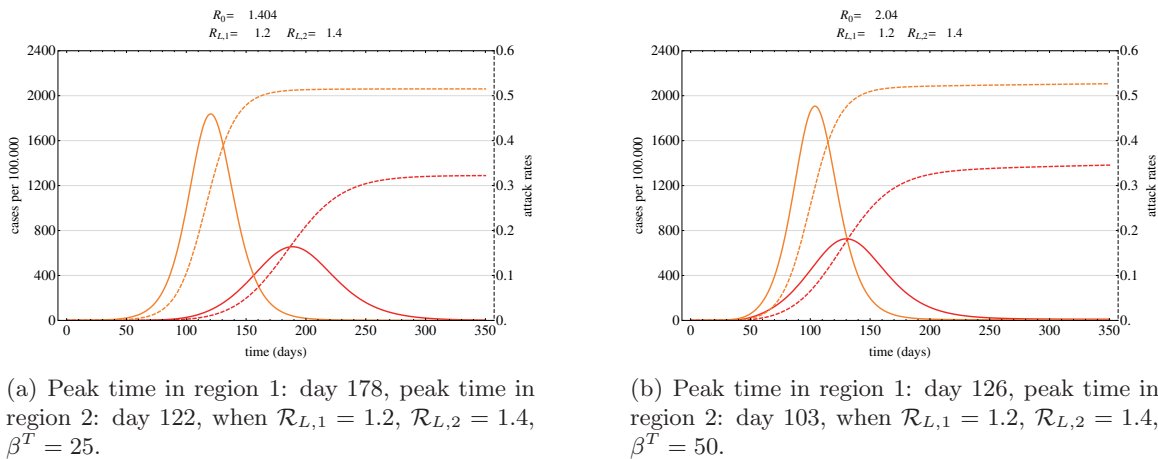
Figure 6. Epidemic curves and attack rates of region 1 (red and red-dashed) and region 2 (orange and orange-dashed) for two values of \beta^T when both the local reproduction numbers are greater than 1. The increase in the value of \beta^T significantly alters the value of \mathcal{R}_0 , but its effect on the epidemic curves only manifests in earlier peak times. Parameter values were chosen as \mathcal{R}_{L,1} = 1.2 , \mathcal{R}_{L,2} = 1.4 , \tau = 0.5 , \mu_E^{-1} = 1.4 , \mu_I^{-1} = 3 , \mu_A^{-1} = 4.1 , p = 0.6 , \rho = 0.1 , \gamma_1^{-1} = \gamma_2^{-1} = 7 , \alpha_1 = 5 \cdot 10^{-5} , \alpha_2 = 5 \cdot 10^{-5} , N_1^I(0) = 3.4 \cdot 10^7 , N_2^I(0) = 3.4 \cdot 10^7 .
