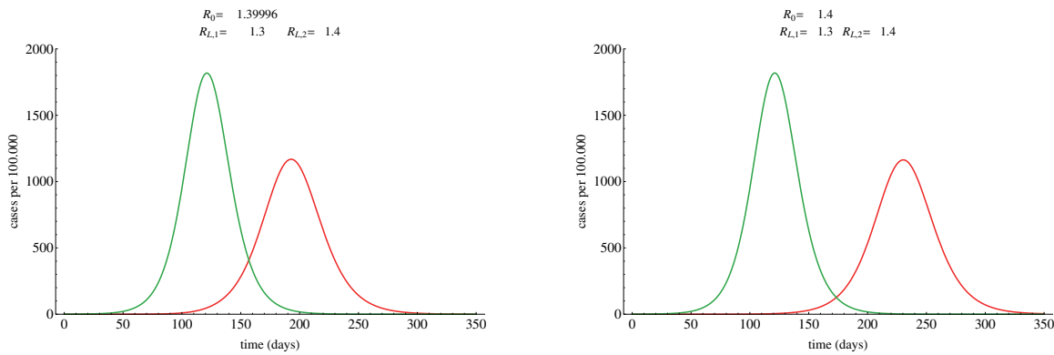
(a) Peak time in Canada: day 195; peak time in Mexico: day 123 when \gamma_1 = \frac{1}{15} , \gamma_2 = \frac{1}{15} .
