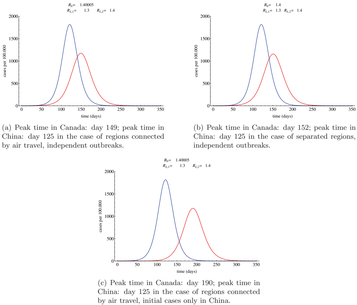
Figure 8. Epidemic curves of Canada (region 1, red) and China (region 2, blue). In the case of independent outbreaks in Canada and China, the effect of travel on the spread of the pandemic is negligible. However, if we assume that the pandemic originates from China and that Canada is susceptible, then due to air transportation the infection invades the disease-free Canada, though with delayed peak time. For the simulations, we set \mathcal{R}_{L,1} = 1.3 , \mathcal{R}_{L,2} = 1.4 , \tau = 0.5 , \gamma_1^{-1} = \gamma_2^{-1} = 7 , \beta^T = 15 , \mu_E^{-1} = 1.4 , \mu_I^{-1} = 3 , \mu_A^{-1} = 4.1 , p = 0.6 , \rho = 0.1 .
